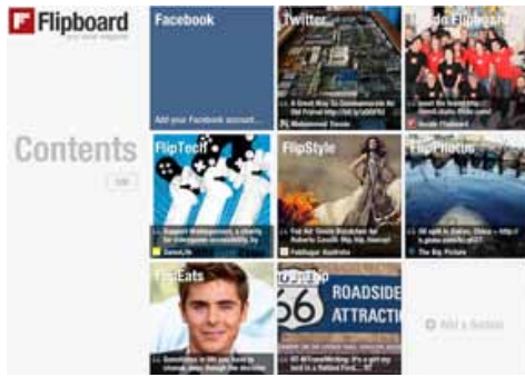
Flipboard interface.
